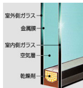
(図3 Low-Eガラス)
